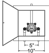
TA-254T-LF
